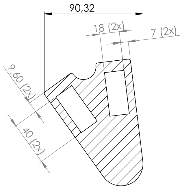
SECTION E-E
